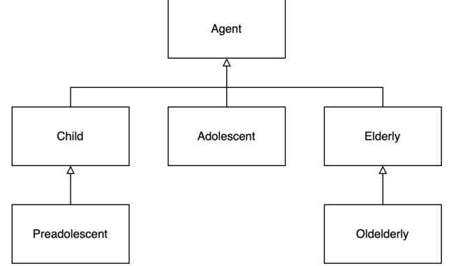
Fig. 1: A simplified UML diagram of class inheritance
